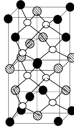
Structure of \text{CuFeS}_2 : Cu (solid), Fe (shaded), S (unfilled).
