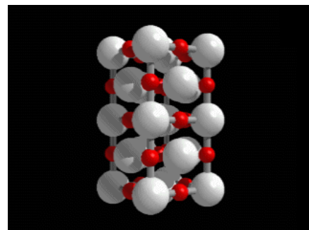
Halite structure of MgO: a FCC arrangement of O^{2-} ions with Mg^{2+} ions filling all octahedral sites.
