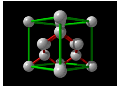
diamond cubic structure in 2 orientations
