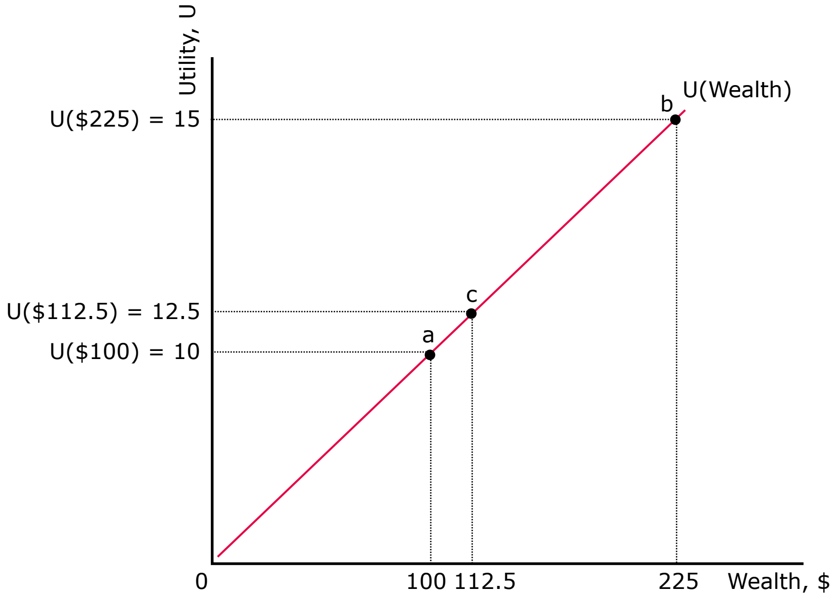
Figure 20-2: Risk neutrality
